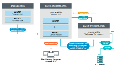
Architecture de la backdoor Gazer
